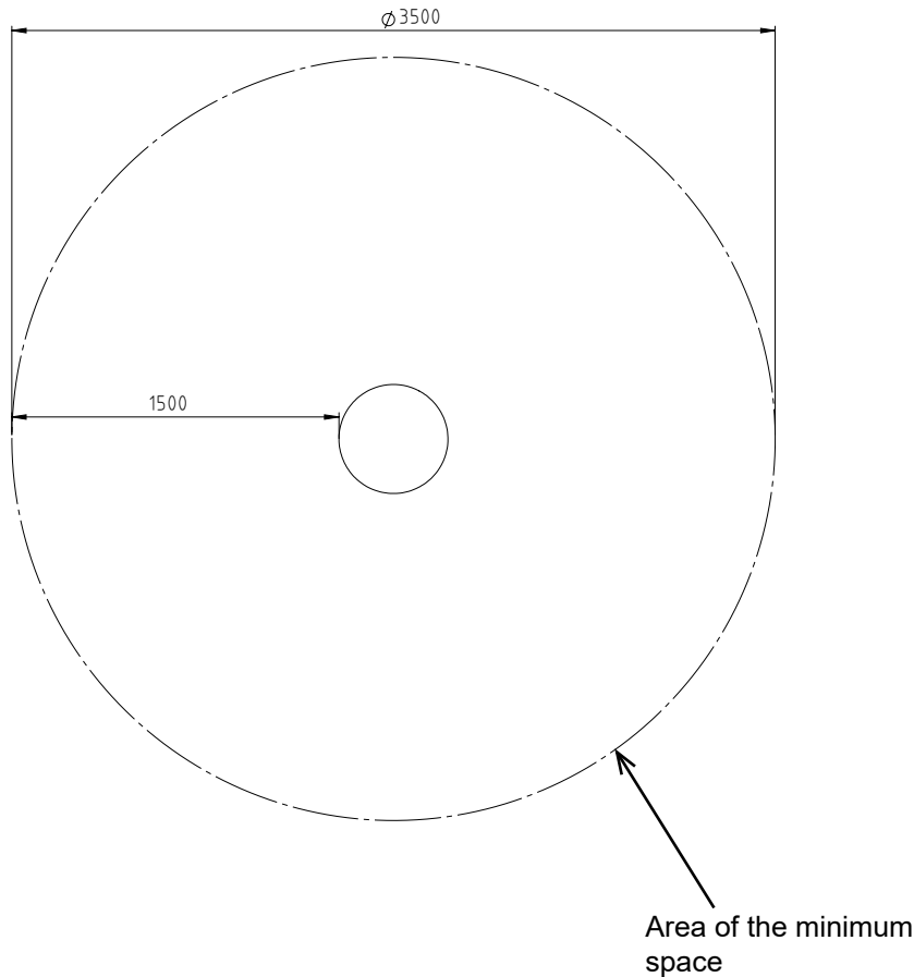
Diagram 3: Top view
